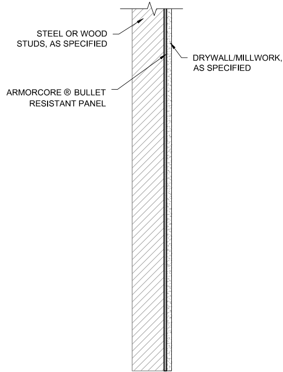
SECTION VIEW
