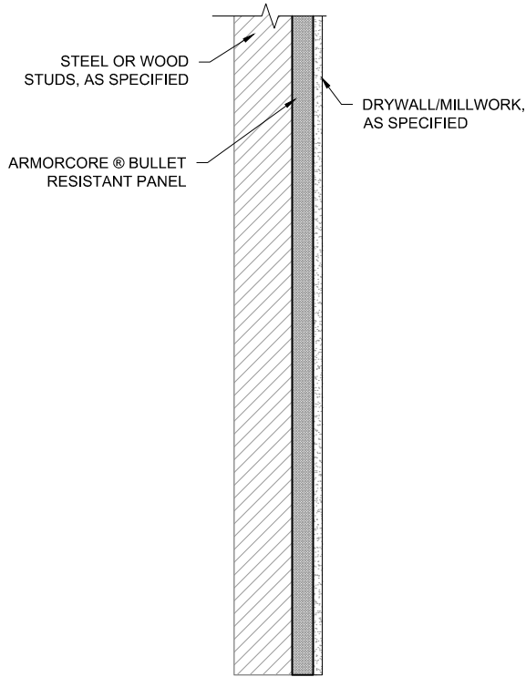
SECTION VIEW
