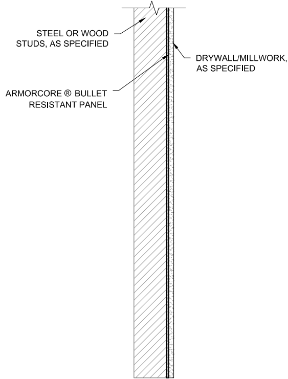
SECTION VIEW
