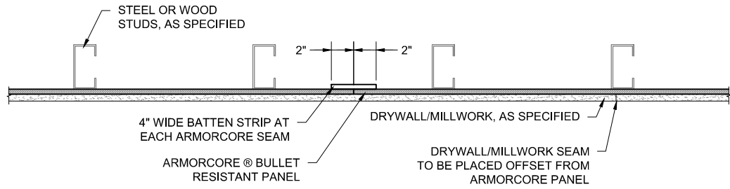
PLAN VIEW
