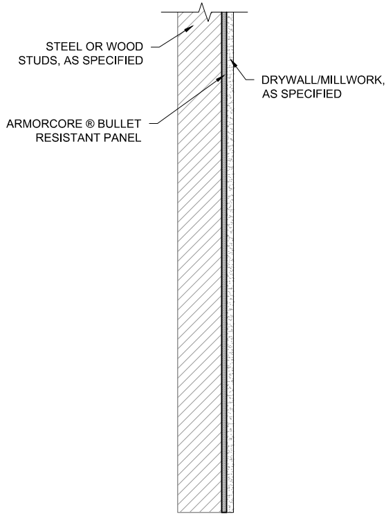
SECTION VIEW
