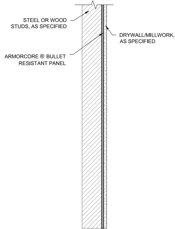
SECTION VIEW
