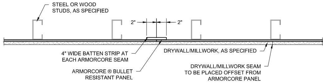
PLAN VIEW
